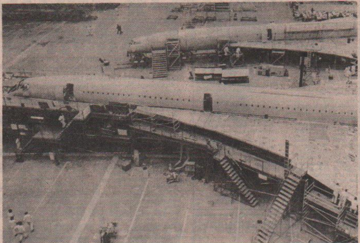
Concorde under construction in Bristol
